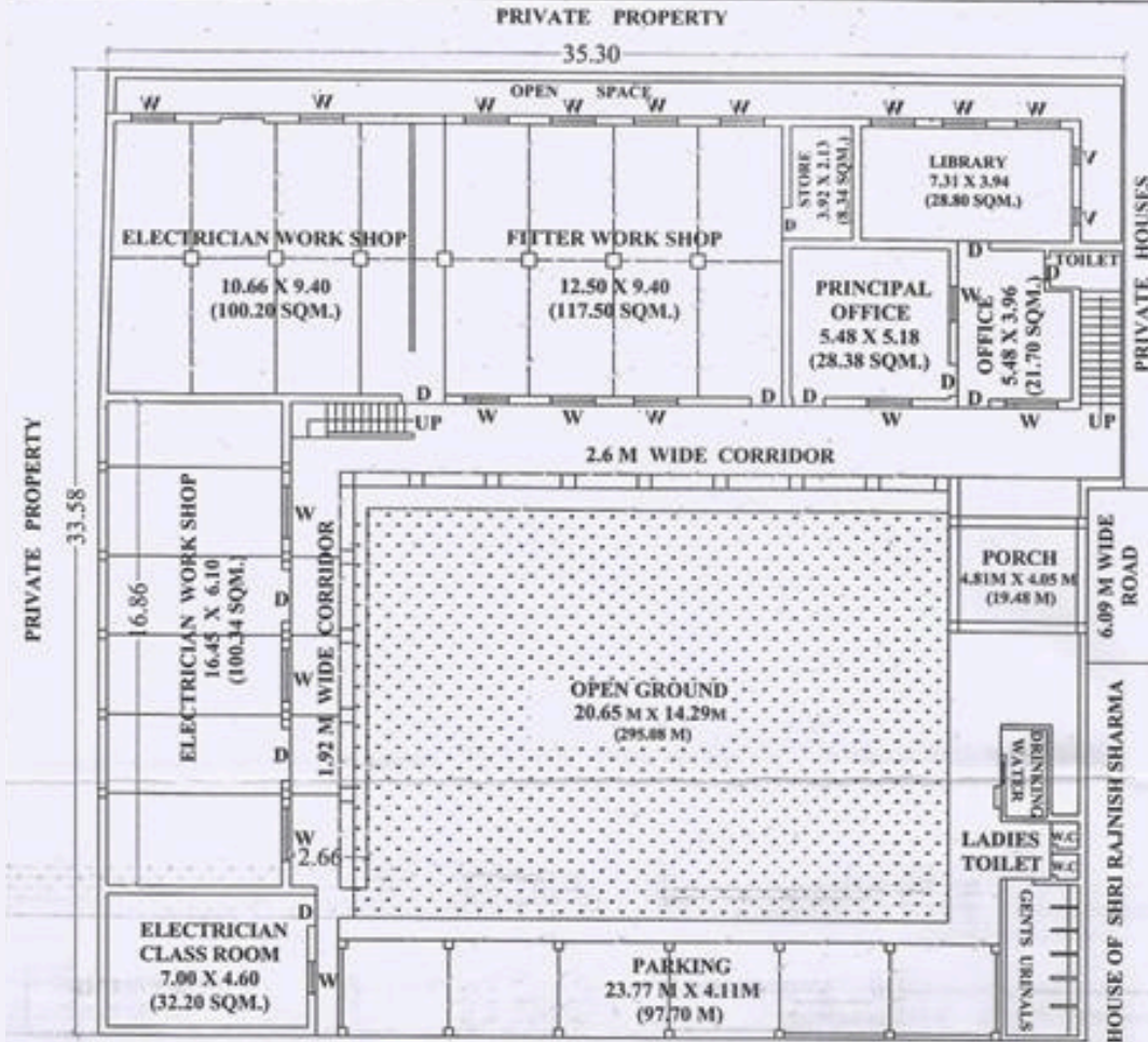
GROUND FLOOR PLAN SCALE :- 1 CM = 5 M
